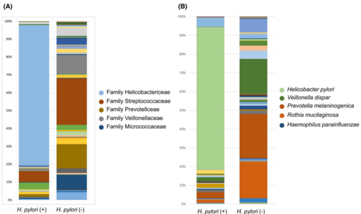
2 FIGURE 3 Relative abundance of gastric microbiota between Helicobacter pylori -positive and H. pylori -negative subjects. At the family level, we observed that Helicobacteraceae accounted for 74.6% of the relative abundance in the H. pylori -positive group. At the species level, H. pylori was the most dominant OTU, accounting for 76.2% of the relative abundance in the H. pylori -positive group
