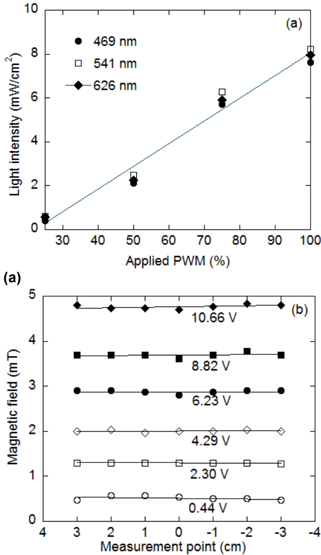
Figure 2. (a) The intensity of LED irradiation at a distance of 2 cm for varying PWM settings; (b) The magnetic field uniformity when the distance between two coils was 6 cm with applied voltage variations.
