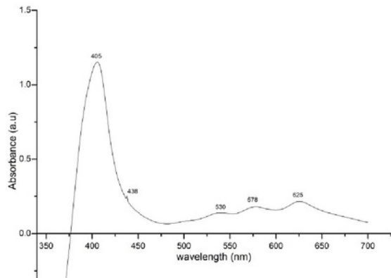
Fig. 5. The absorption spectrum of chlorophyll.
