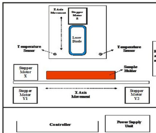
Fig. 1. The schematic CNC laser for irradiation treatment
