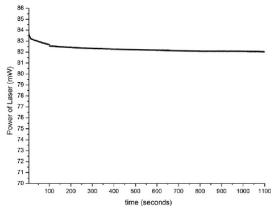
Fig. 3. The steady state of Power of Laser.
