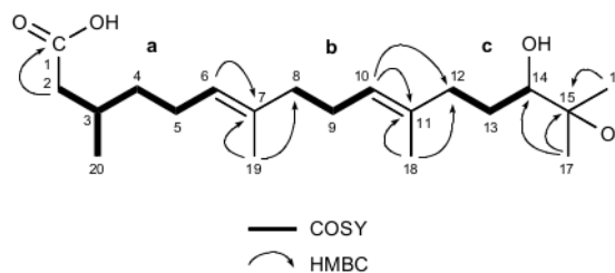
Figure 2: Selected 2D NMR Correlations for Melidianolic Acid B ( 2 ).
