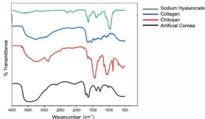
Figure 1. FTIR Spectra
