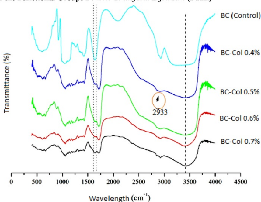
Fig. 1. Comparison of the IR spectra of Samples.
