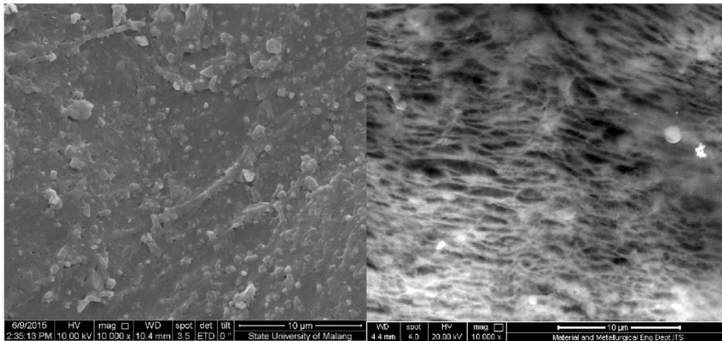
Fig. 3. (a) Sample Surface (Cross Section Area) Bacteria Cellulose-Collagen Control with a magnification of 10.000X (b) Surface (Cross Section Area) Bacteria Cellulose-Collagen 0.4% with a magnification of 10.000X.
