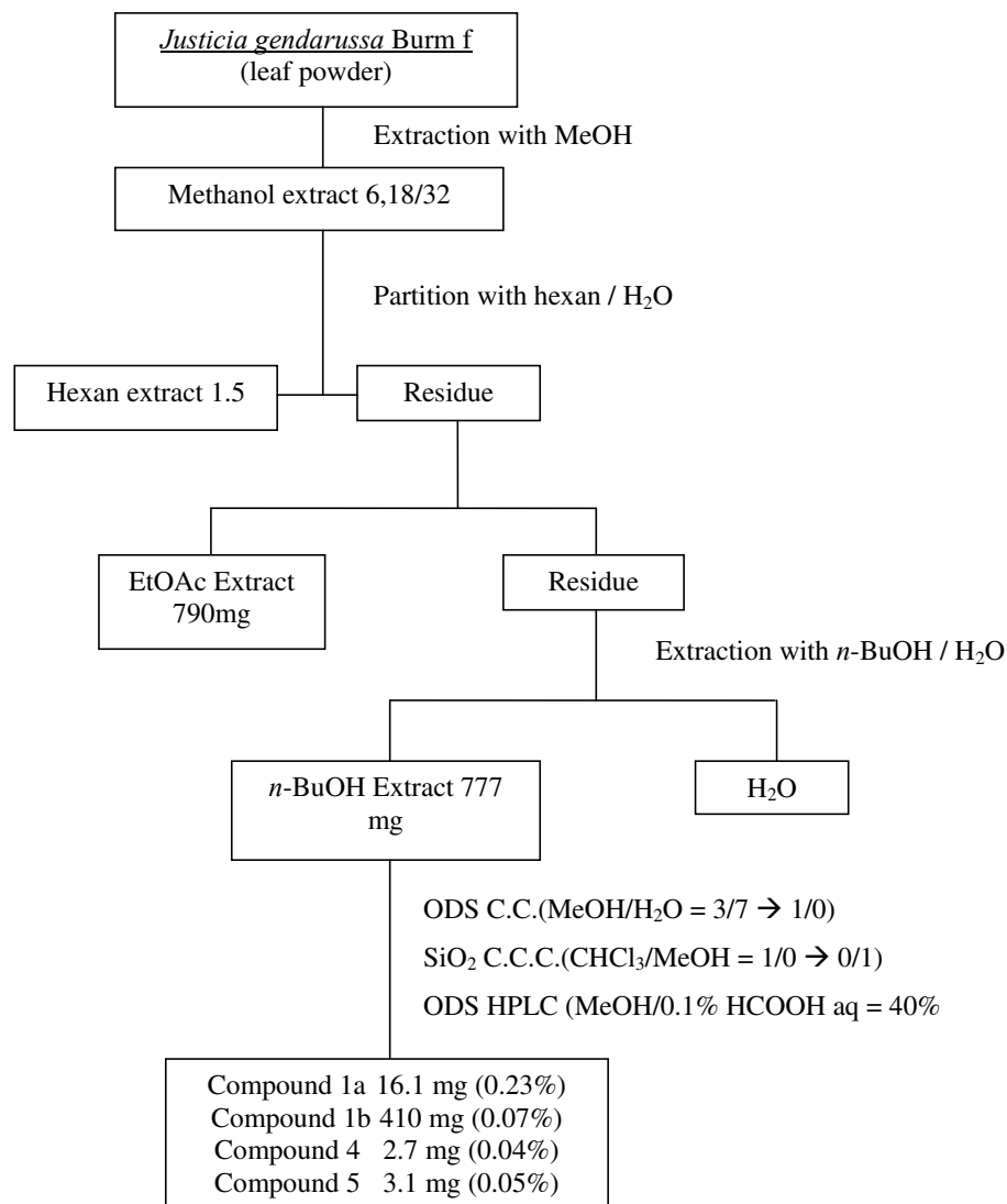
Figure 1. Scheme of flavonoids isolation
