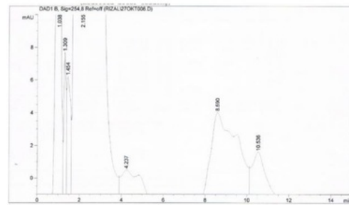
Gambar 5. Kromatogram Standar Gendarusin A 9,6 ppm
