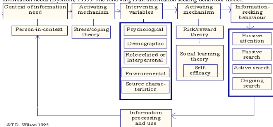
Figure 6: A revised general model of information behaviour
