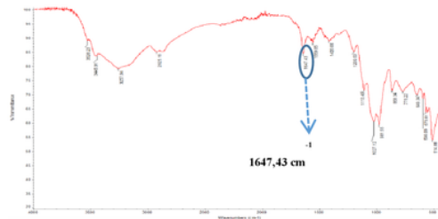
Figure 2. Fourier Transform Infrared (FTIR) Result
