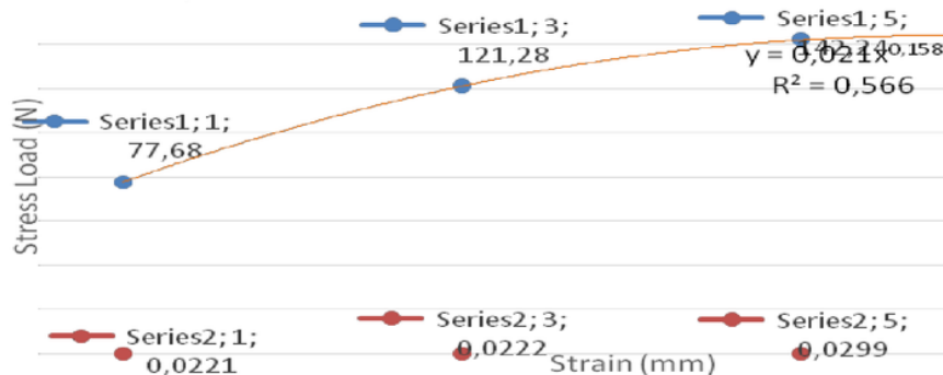
Figure 2. Composite Tensile Test Results
