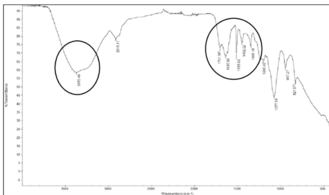
Figure 6. IR Spectrum of Hydrogel With Variations of HA-PEG-0 HRP
