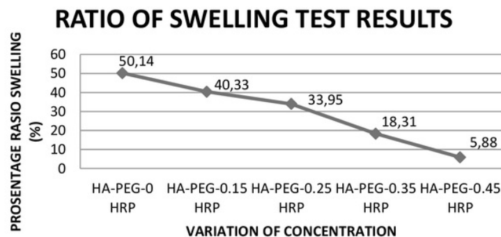
Figure 2. Line Graph of Swelling Test Results
