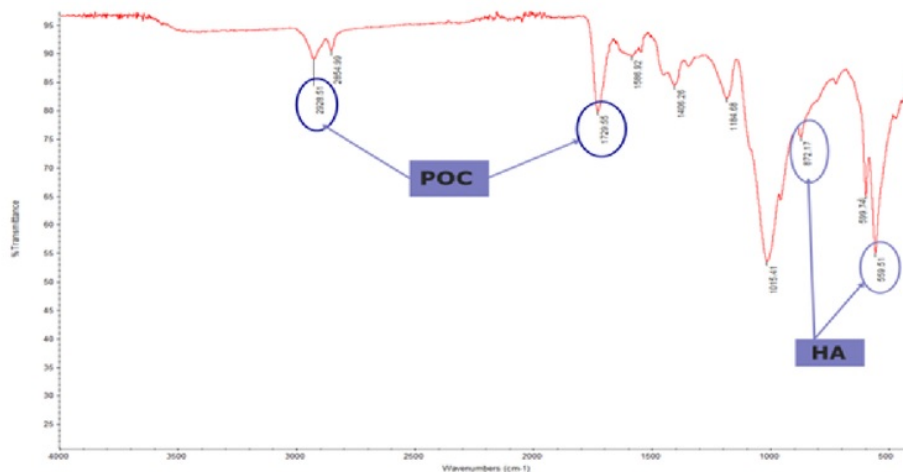
Figure 2. POC-HA composite IR spectrum
