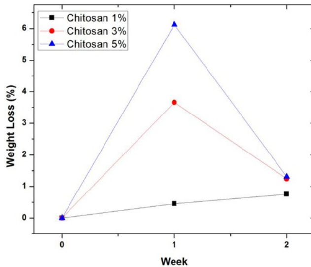
Figure 5. The result of degradation test
