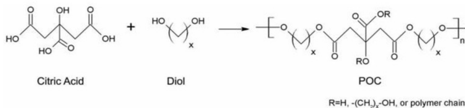
Figure 1. Chemical reaction of POC synthesis
