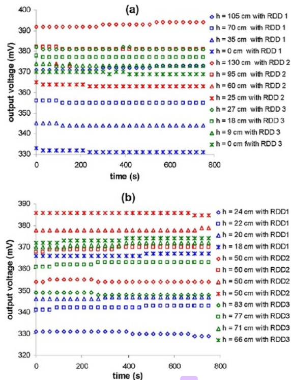
Fig. 8. Sensor stability curve for the area of (a) front slope and (b) back slope.
