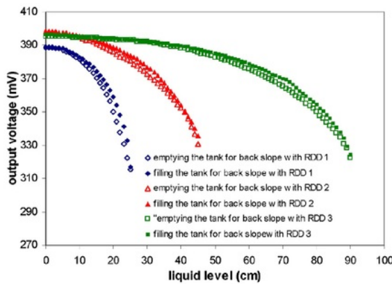
Fig. 6. Back slope curve of the liquid level sensor.
