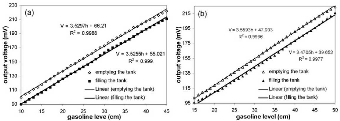
Fig. 4. The linear region of output voltage detector to gasoline level for (a) RDD A and (b) RDD B.
