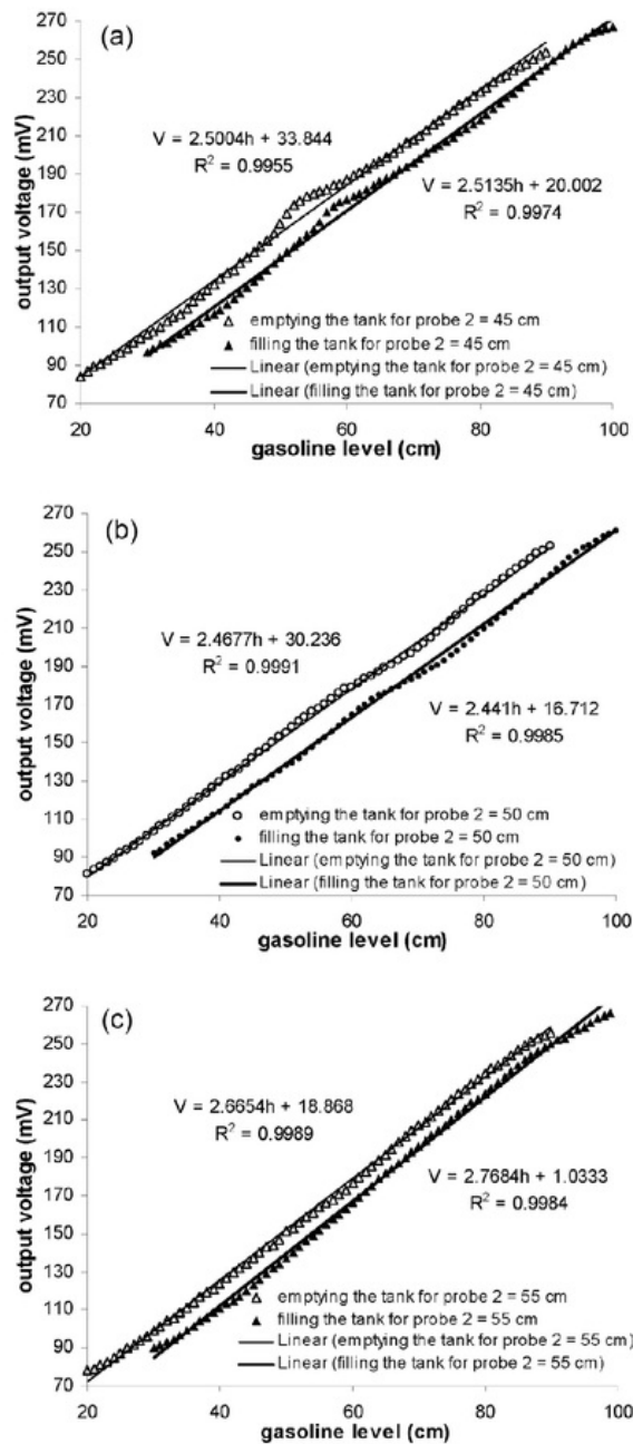
Fig. 7. Linear graph of the relationship between the output voltage detector to the level of gasoline for (a) position of the probe 2 = 45 cm, (b) position of the probe 2 = 50 cm, and (c) position of the probe 2 = 55 cm.
