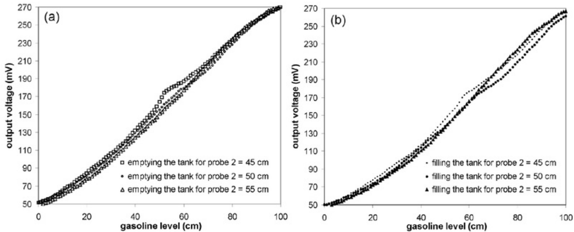
Fig. 6. Comparison chart data for probe 2 position of 45 cm, 50 cm, and 55 cm above probe 1 in process of (a) emptying and (b) filling.
