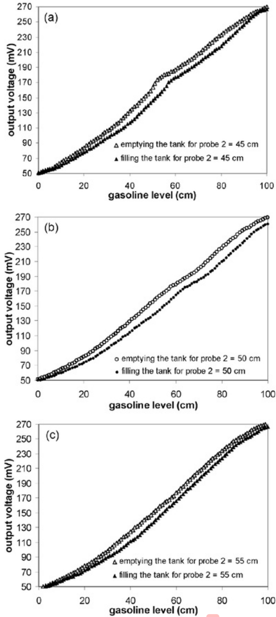
Fig. 5. Plot the data output voltage detector vs. gasoline level for emptying and filling process with position of probe 2 (a) 45 cm (b), (c) and 55 cm above probe 1.
