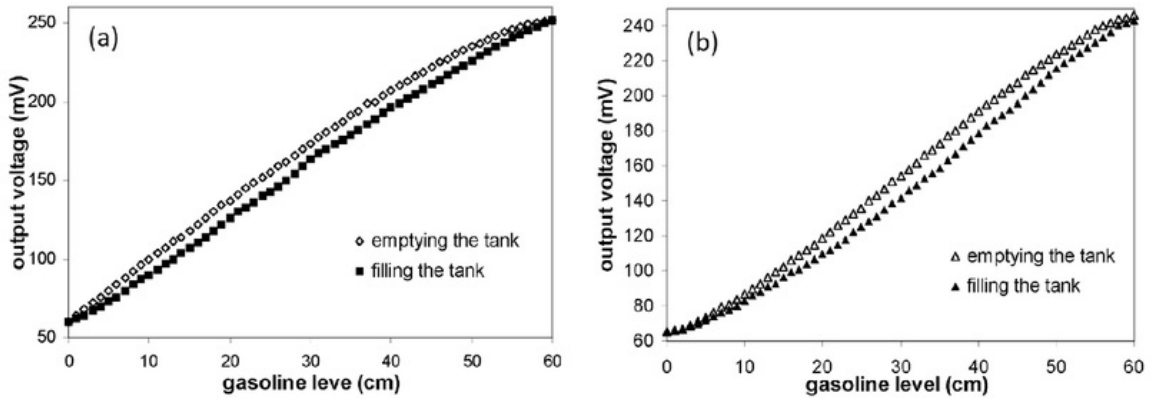
Fig. 3. Plot of output voltage detector to the gasoline level for (a) RDD A and (b) RDD B.
