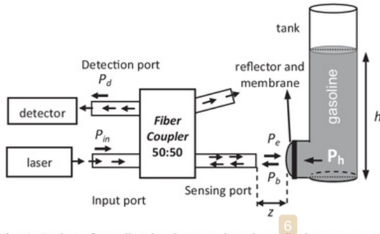
Fig. 1. Design of gasoline level sensor based on displacement sensor using fiber coupler.
