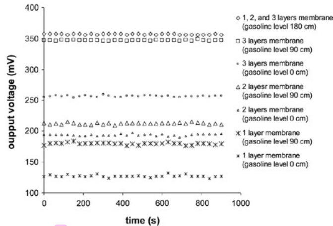
Fig. 7. The plot of detector output voltage as a function of time duration of sensor stability test.
