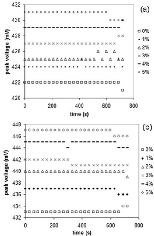
Fig. 7. Stability of the sensor for (a) CM 1 and (b) CM 2.
