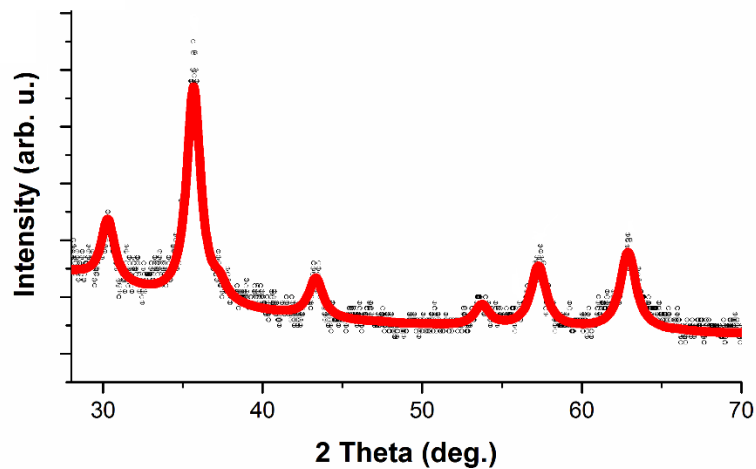
Figure 2. XRD pattern of the dried \text{Fe}_3\text{O}_4 fluid at room temperature
