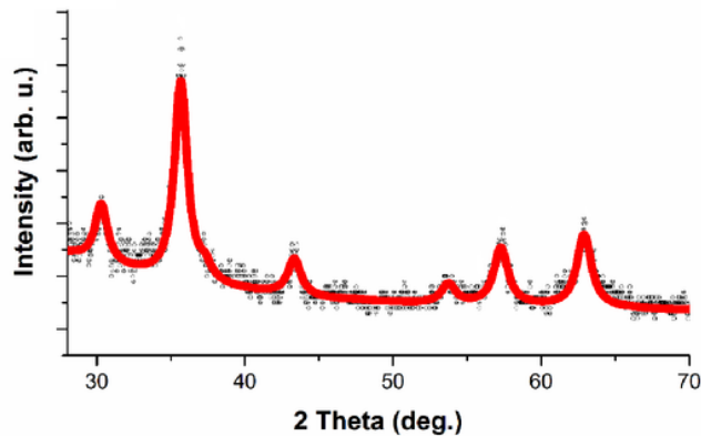
Figure 2. XRD pattern of the dried Fe 3 O 4 fluid at room temperature
