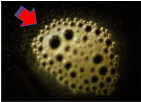
Fig 1. Catalase test on Staphylococcus aureus shows positive bubbles
