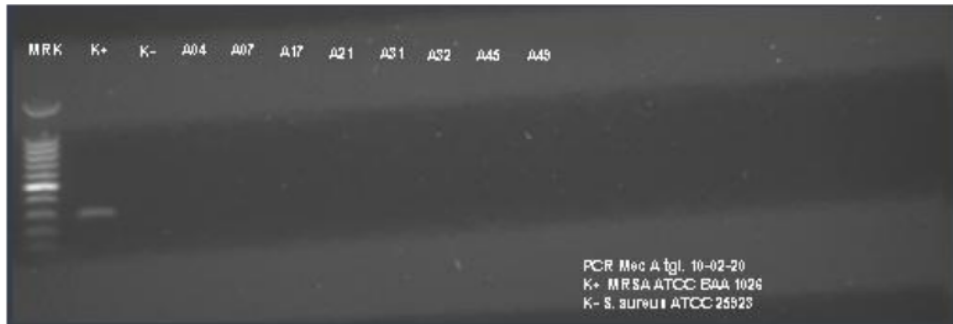
Figure 4. Meca PCR results with positive bands at 310 bp. MRK Line: 100-bp molecular-weight markers, Line K +: MRSA ATCC BAA 1026 (Positive Control), Line K-: Staphylococcus aureus ATCC 25923 (Negative Control), Line A04-A49: Negative isolate for mecA gene
