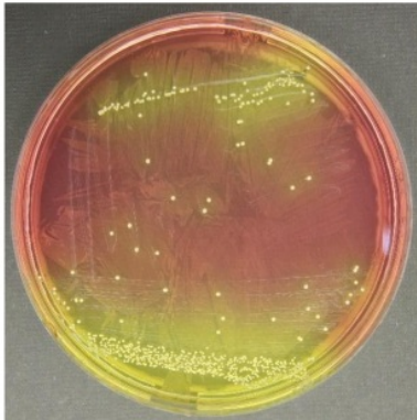
Figure 1. The results of positive yellow Mannitol Fermentation and S. aureus colonies appear mucoid white on Mannitol Salt Agar medium (HiMedia Pvt. Ltd, M118) (Canon 600D DSLR). 72 x 72 dpi
