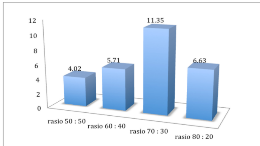
Fig. 5 Compressive strength value of scaffold CA:Ch-GEL
