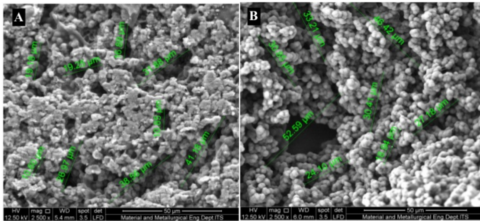
Fig. 6 The results of SEM CA:Ch-GEL scaffold with ratio 50:50 (A), ratio 60:40 (B) at 2500x magnification
