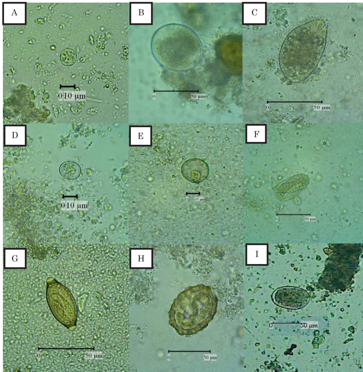
Figure 2. Morphology of Gastrointestinal Parasites in Pig in Bali Province Under Light Microscope. A). Entamoeba sp. (Bar: 10µm); B) and C). Balantidium sp. Cyst and Trophozoite (Bar: 50µm); D). Eimeria sp. (Bar: 10µm); E). Blastocystis sp. (Bar: 10µm); F). Strongyloides sp. (Bar: 50µm); G). Trichuris sp. (Bar: 50µm); H). Ascaris sp. (Bar: 50µm); and I). Oesophagostomum sp. (Bar: 50µm).
