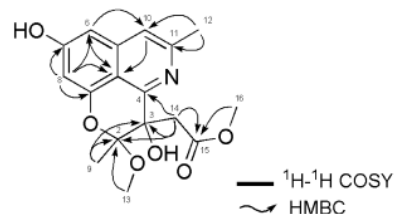
Fig. 4. Selected 2D-NMR Correlations for Cassiarin J (3)
