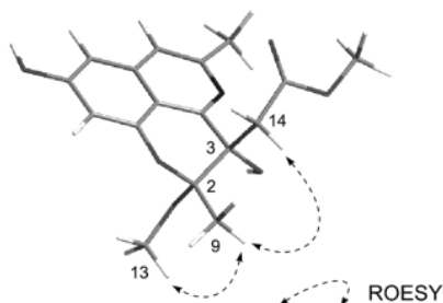
Fig. 5. Most Stable Conformation of Cassiarin J (3) by Monte Carlo Conformational Search and the Selected ROESY Correlations
