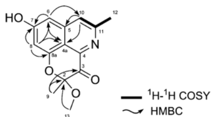
Fig. 1. Selected 2D-NMR Correlations for Cassiarin G (1)
