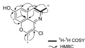
Fig. 6. Selected 2D-NMR Correlations for Cassiarin K (4)
