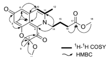
Fig. 3. Selected 2D-NMR Correlations for Cassiarin H (2)
