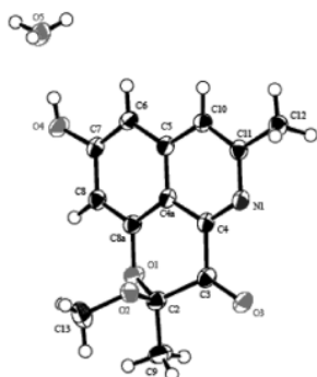
Fig. 2. An ORTEP Drawing for Cassiarin G (1)
