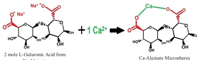
FIGURE 3. Simulation of a reaction between the alginic acid carboxylic group and \text{Ca}^{2+}
