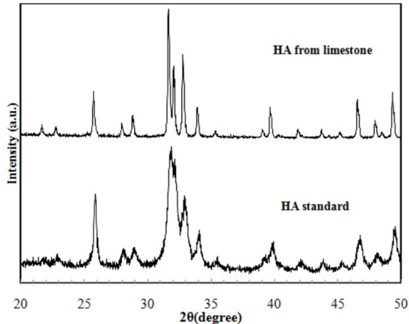
Fig. 2 : Comparison of XRD patterns between hydroxyapatite from Padalarang and Cirebon limestone(top) and hydroxyapatite standard (bottom).
