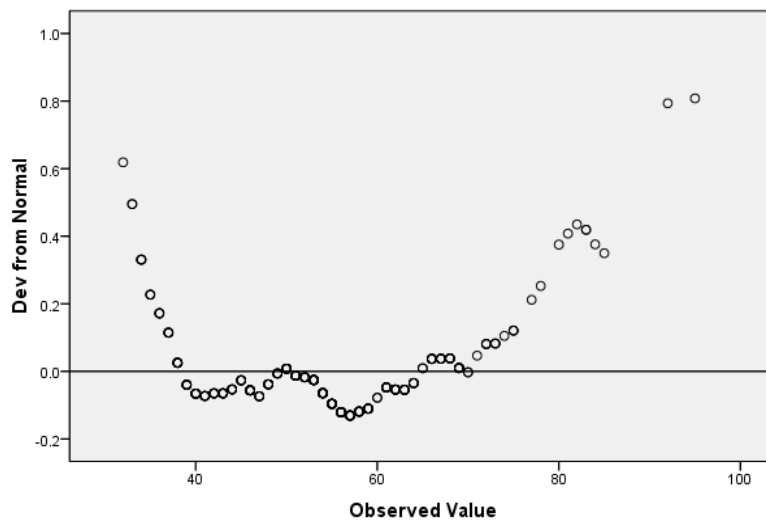
Detrended Normal Q-Q Plot of VarY
