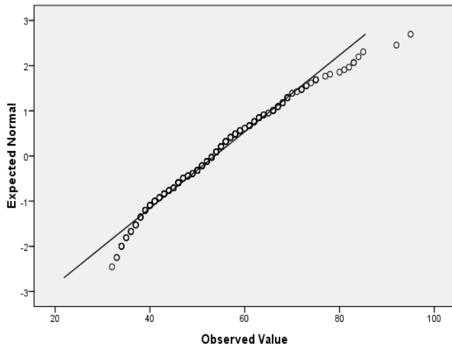
Normal Q-Q Plot of VarY
