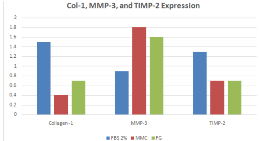
Fig. 5 : Collagen-1, MMP-3 and TIMP-2 Expression among groups.
