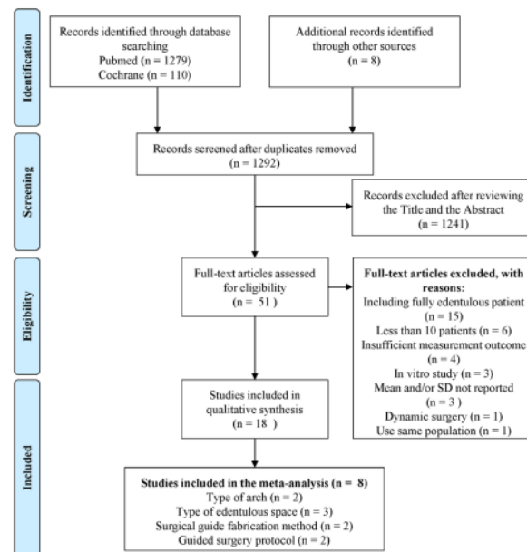
Fig. 2. Flow diagram of articles found through databases.
