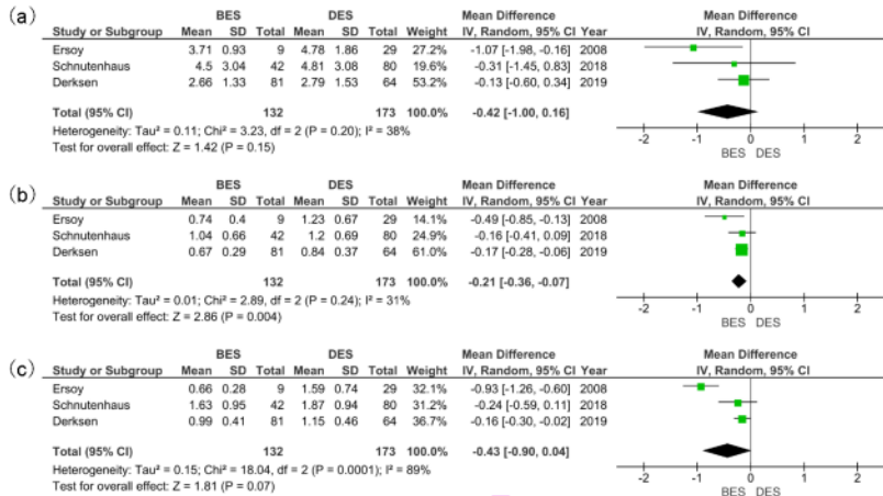
Fig. 6. Forest plot evaluating the effects of edentulous space (BES vs DES); (a) angular deviation; (b) coronal deviation; and (c) apical deviation.
