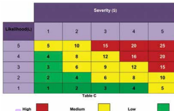
Figure 3: Risk Matrix
