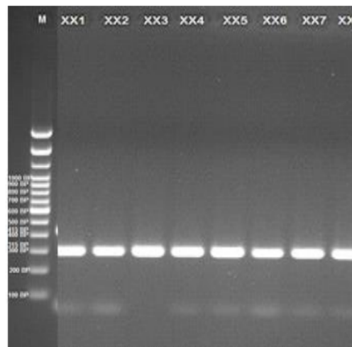
Fig. 4 The PCR results of female sexing Limousine cattle spermatozoa (XX) (415 bp)
