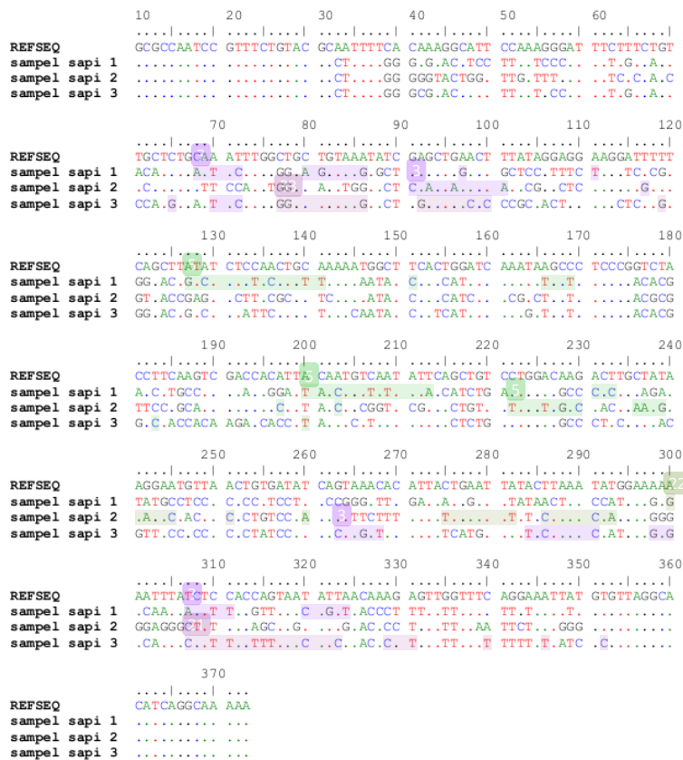
Gambar 2. Urutan nukleotida gen rLH. Refseq = Genbank, sampel sapi 1 = Sapi Madrasin, sampel sapi 2 = Sapi Madura, sampel sapi 3 = Sapi Limousin.
