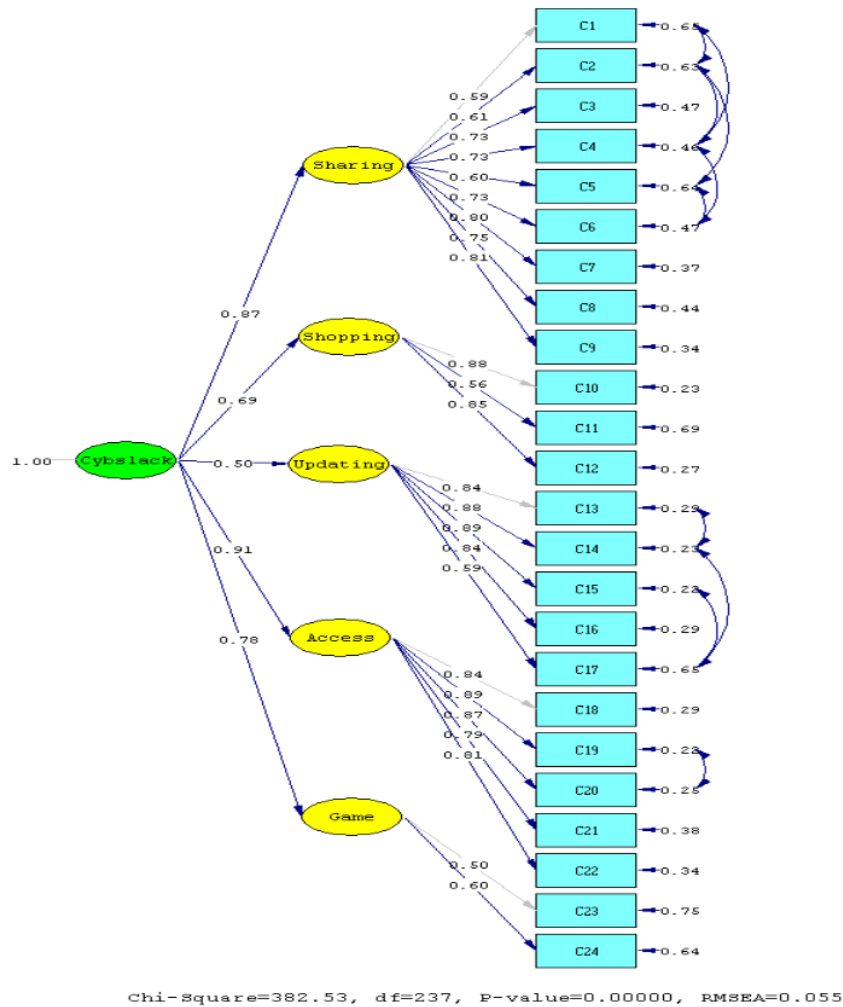
Gambar 1. Second Order CFA Adopsi Skala Cyberslacking
