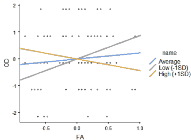
Gambar 2. Simple slope plot X, Z, Y 2
