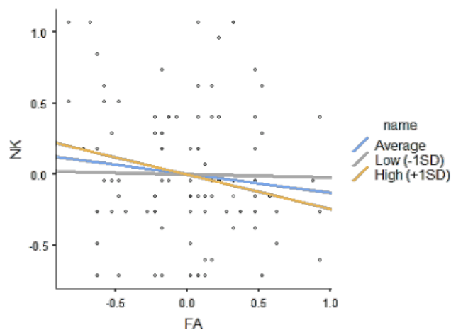
Gambar 1. Simple slope plot X, Z, Y 1
