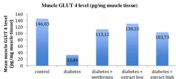
Figure 2. GLUT levels of 4 gastrocnemius muscles after treatment.
