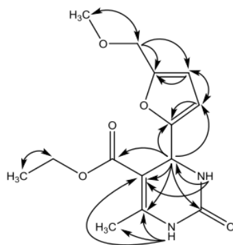
Figure 3. Selected HMBC correlation for compound 4.
