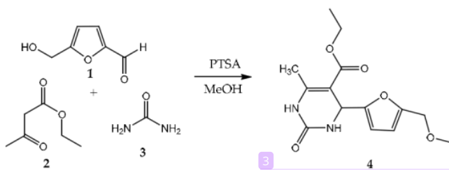
Scheme 1. Synthesis of ethyl 4-[5-(methoxymethyl)furan-2-yl]-6-methyl-2-oxo-1,2,3,4-tetrahydropyrimidine-5-carboxylate (4).
