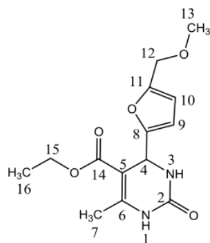
Figure 1. Numbering of the title compound.
