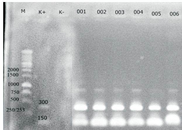
Figure 1. Results of agarose gel electrophoresis.
