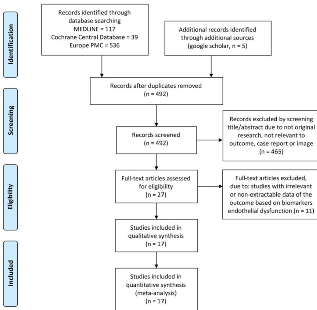
Fig. 1. PRISMA flowchart.
