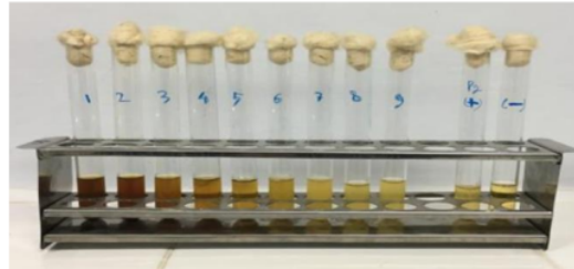
Figure 1. Results of serial dilution of okra extract on P. gingivalis bacteria by observing the turbidity and obtained MIC on the 6th tube and MBC on the 5th tube.
