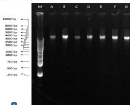
8 Figure 1. Total DNA Electrophoresis Results in 1% agarose. M:marker; A-F: sampel code
