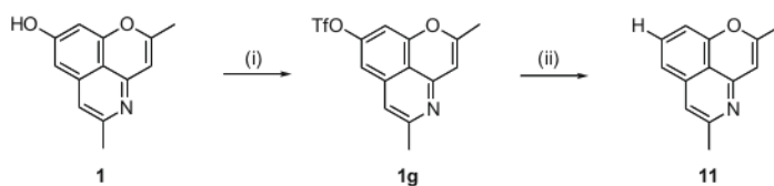
Scheme 3. Synthesis of 1g and 11 . Reagents and conditions: (i) Tf 2 O, pyridine, CH 2 Cl 2 , rt; (ii) TES, Pd(PPh 3 ) 2 Cl 2 , DMF, reflux.
