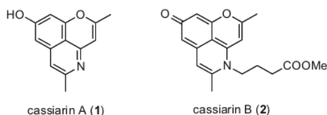
Chart 1. Structures of cassiarins A ( 1 ) and B ( 2 ).
