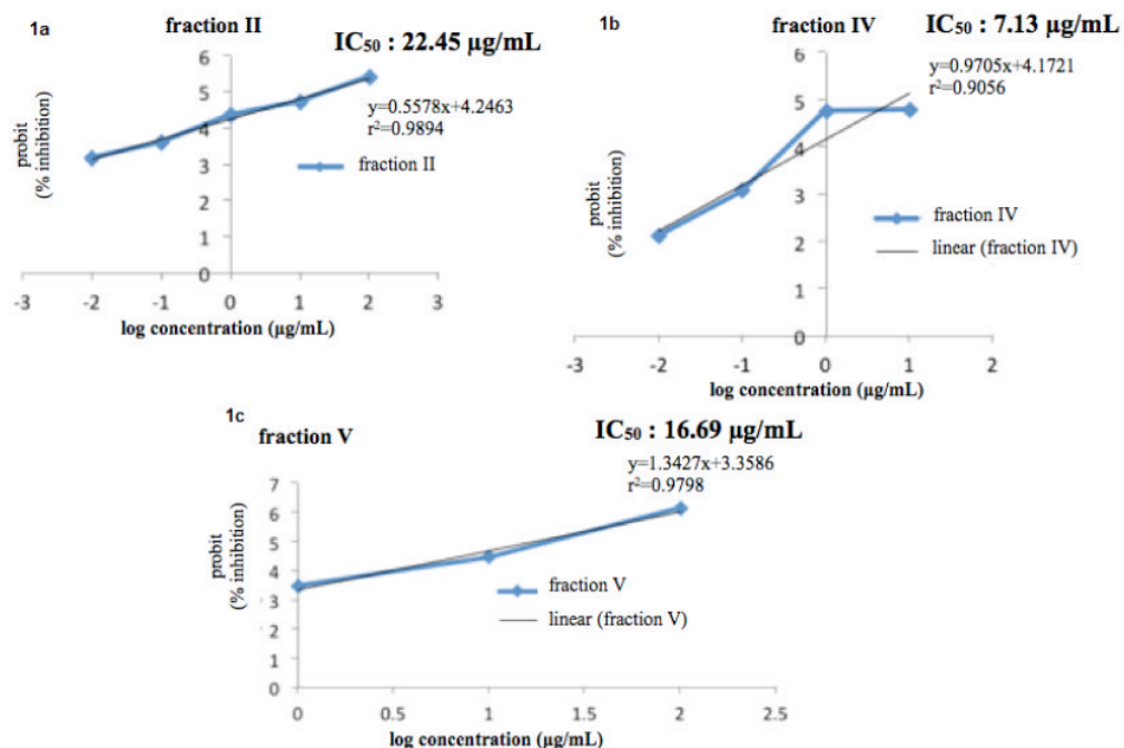
Fig 1. Percentage inhibition of the three fractions against Plasmodium falciparum , fraction II: IC 50 22.45 µg/mL; IV: IC 50 7.13 µg/mL; and V: IC 50 16.69 µg/mL
