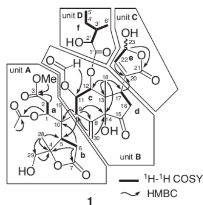
Figure 1. Selected 2D NMR correlations for 1
