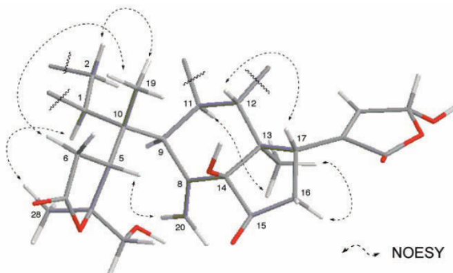
Figure 3. Selected NOESY correlations and relative configurations for 1
