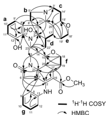
Fig. 2 Selected 2D NMR correlations of 1
