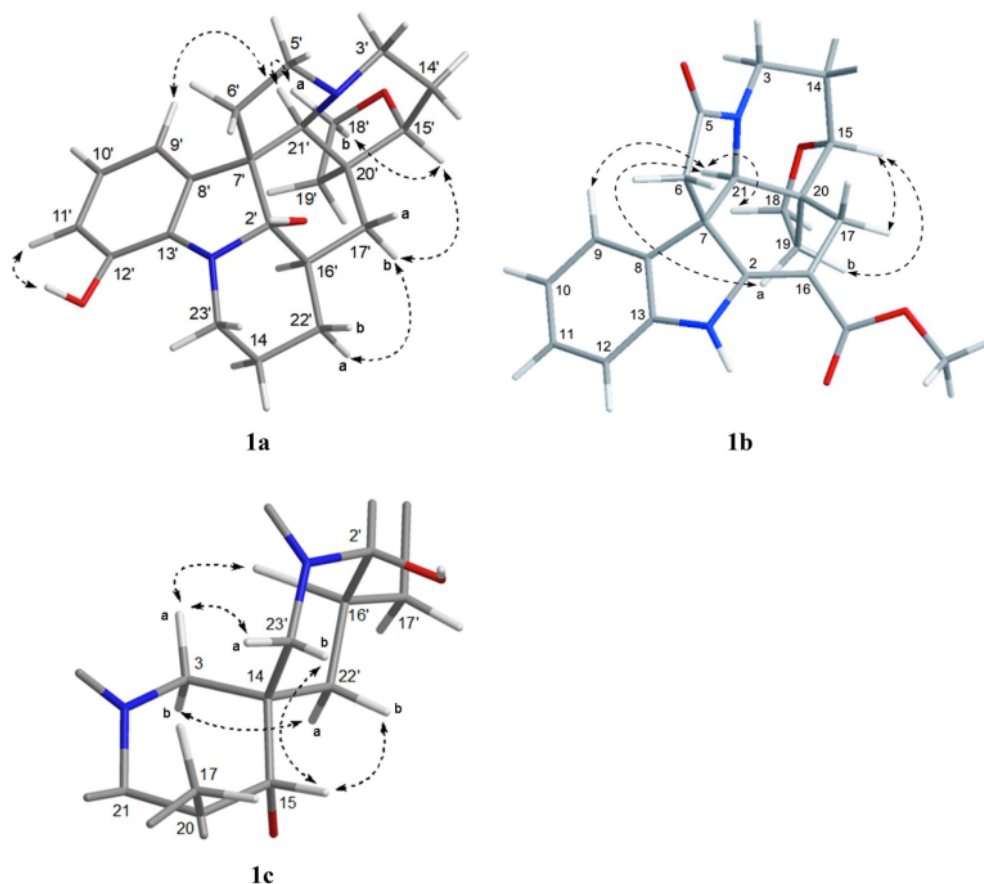
Fig. 3 Selected NOESY correlations of 1
