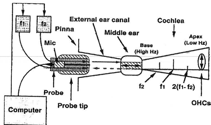
Figure 1. DPOAE examination tools and procedures. 14
