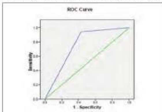
Fig. 2 - ROC curve
