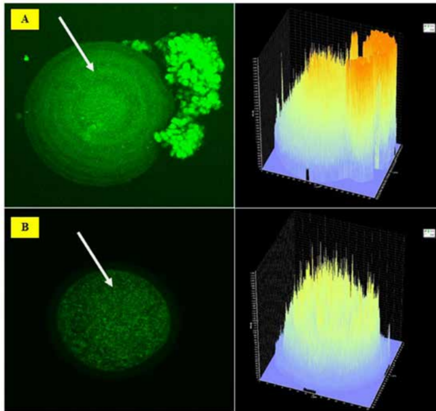
Fig. 2. Calcium intensity ( Ca^{2+} ) in COC after vitrification was concentrated in the nucleolus (B), in fresh COC without vitrification it was concentrated in the cytoplasm (A); White arrows: COCs are in good condition, and arrows show fluorescent luminescence in the nucleus and cytoplasm (Olympus Microscope, Japan Type FV1000, Olympus Software FLUoview version 4.2a; x100).
