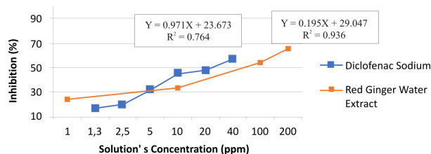
Fig. 1. Differences percentage inhibition of bovine serum albumin in vitro due to diclofenac sodium (positive control) and red ginger water extract
