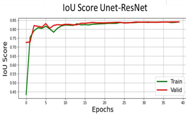
Fig. 6. IOu Score UNet-ResNet34 Architecture
