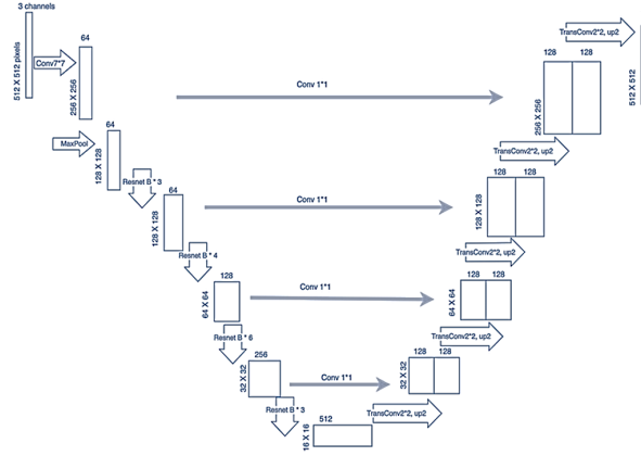
Fig. 3. UNet Architecture with ResNet Encoder
