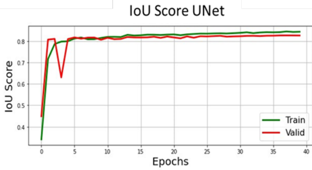
Fig. 4. IOu Score UNet Architecture
