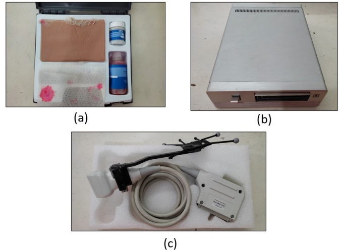
Fig. 1. (a) Phantom human body part standart, (b) USG modality Telemed SmartUs EXT-1M, and (c) Linear Probe type L15-7L40H-5.
