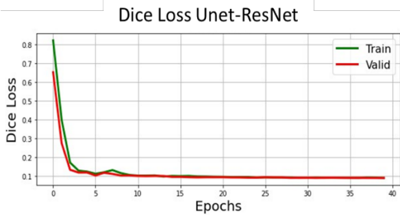
Fig. 7. Dice Loss UNet-ResNet34 Architecture
