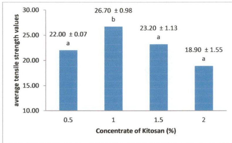
Figure 3. Histogram of average tensile strength values
