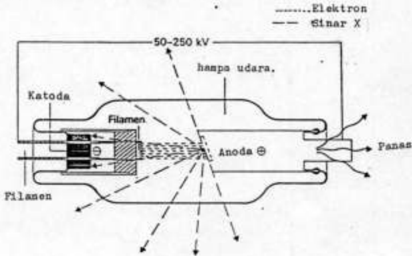
Gambar 1. Tabung sinar X tipe Anoda statis . ( Sumber : Chesney, 1984 )
